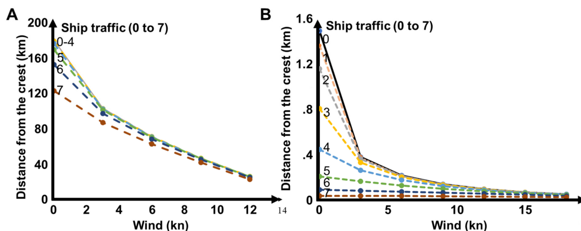
Figure 6. Detection distance of (A) the individual sounds represented as the 90th percentile with 10 dB above the Wenz background noise ( Q_{0.90} - 10 ) between 570 and 2000 Hz (B) and fish ambient noise level (ANL) as a function of the wind in knots. The solid line is without considering boats and dashed lines are when considering ship traffic from the Wenz model; each colour corresponds to a ship traffic regime also numbered from 1 (upper line) to 7 (bottom line).
